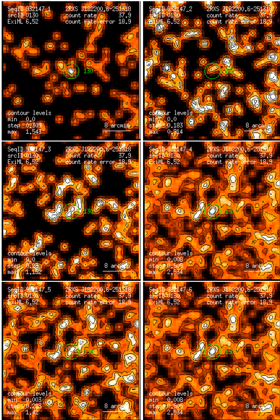
Figure 130: RASS 932147: detection 0130: band rate images, Gaussian filter: (1) PSPC channels 11 – 41, (2) 52 – 90, (3) 91 – 201, (4) 11 – 235, (5) 52 – 201, (6) 11 – 201. Broad band rates in counts/ks. Band rate contour levels in counts/ks/arcmin 2 .
