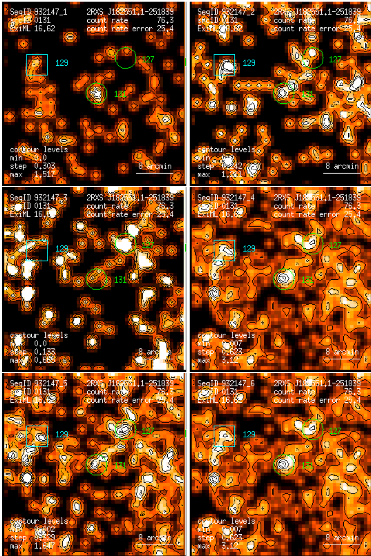
Figure 131: RASS 932147: detection 0131: band rate images, Gaussian filter: (1) PSPC channels 11 – 41, (2) 52 – 90, (3) 91 – 201, (4) 11 – 235, (5) 52 – 201, (6) 11 – 201. Broad band rates in counts/ks. Band rate contour levels in counts/ks/arcmin 2 .
