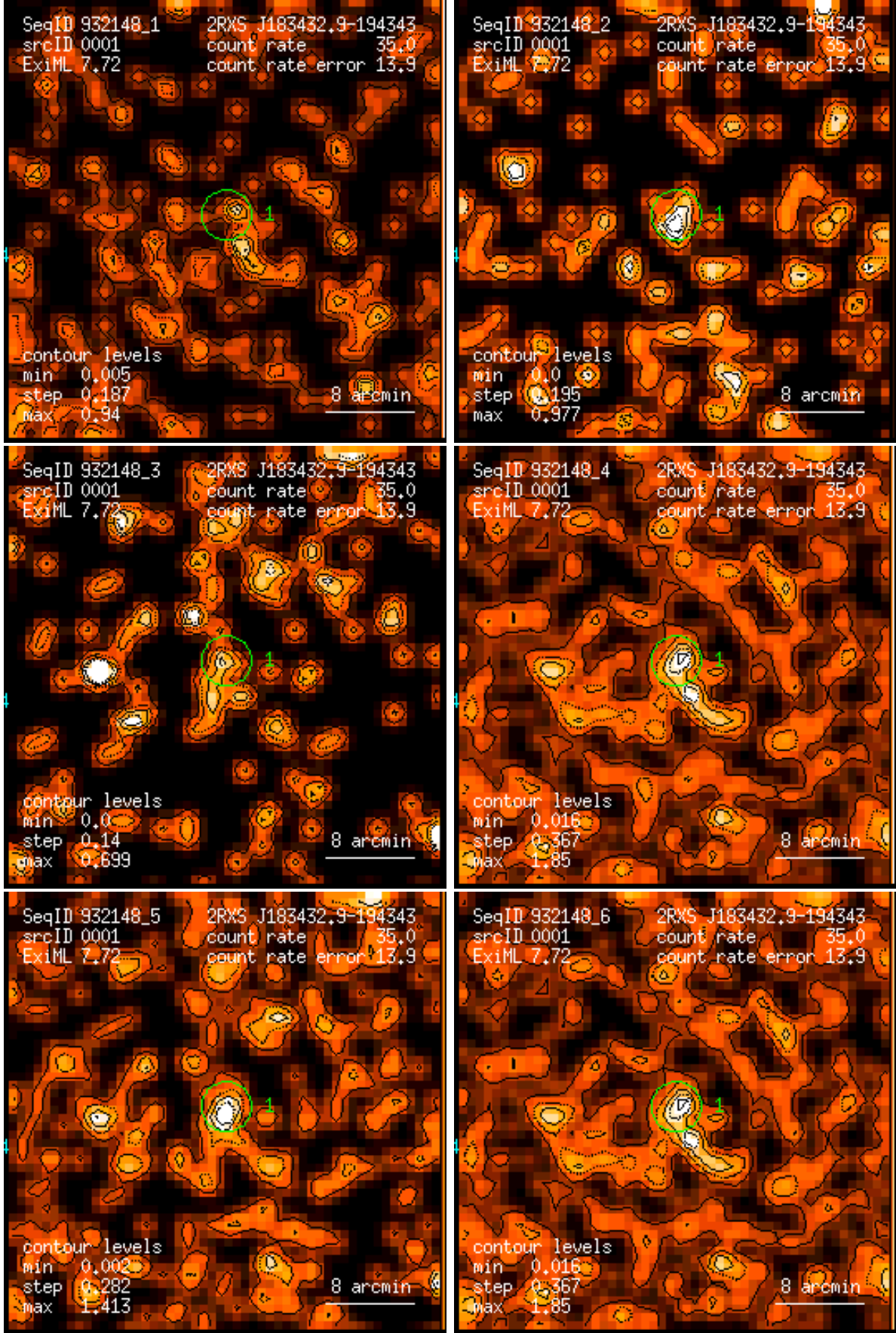
Figure 1: RASS 932148: detection 0001: band rate images, Gaussian filter: (1) PSPC channels 11 – 41, (2) 52 – 90, (3) 91 – 201, (4) 11 – 235, (5) 52 – 201, (6) 11 – 201. Broad band rates in counts/ks. Band rate contour levels in counts/ks/arcmin 2 .
