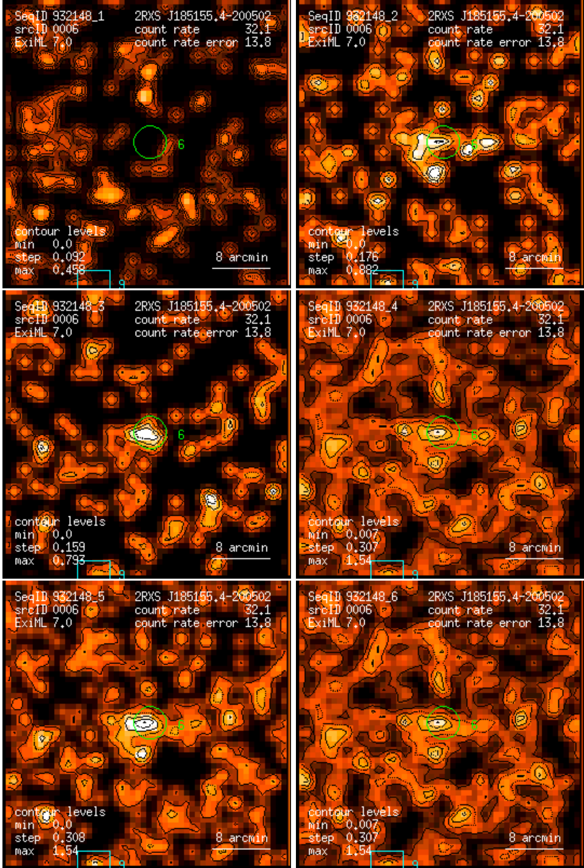
Figure 6: RASS 932148: detection 0006: band rate images, Gaussian filter: (1) PSPC channels 11 – 41, (2) 52 – 90, (3) 91 – 201, (4) 11 – 235, (5) 52 – 201, (6) 11 – 201. Broad band rates in counts/ks. Band rate contour levels in counts/ks/arcmin 2 .
