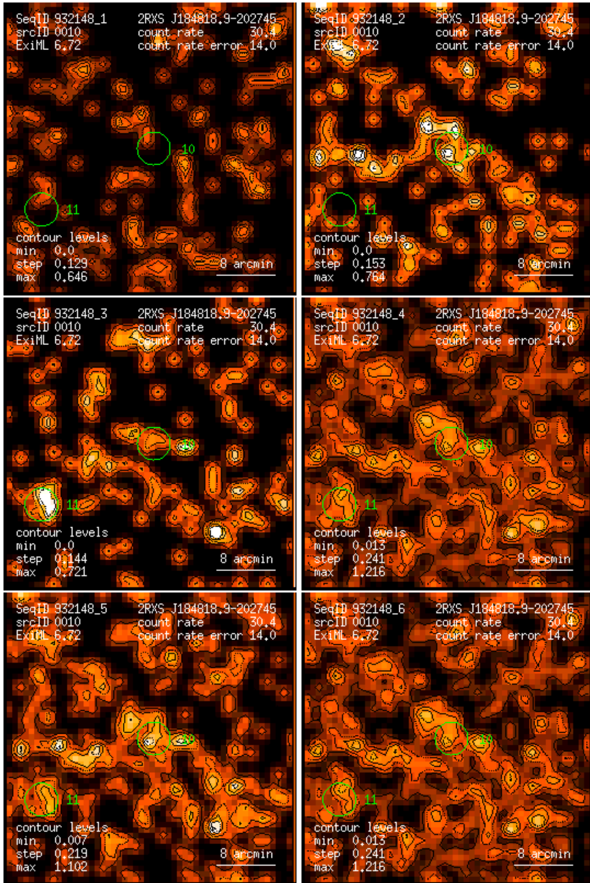
Figure 10: RASS 932148: detection 0010: band rate images, Gaussian filter: (1) PSPC channels 11 – 41, (2) 52 – 90, (3) 91 – 201, (4) 11 – 235, (5) 52 – 201, (6) 11 – 201. Broad band rates in counts/ks. Band rate contour levels in counts/ks/arcmin 2 .
