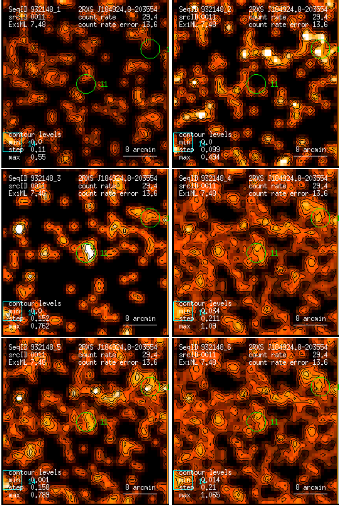
Figure 11: RASS 932148: detection 0011: band rate images, Gaussian filter: (1) PSPC channels 11 – 41, (2) 52 – 90, (3) 91 – 201, (4) 11 – 235, (5) 52 – 201, (6) 11 – 201. Broad band rates in counts/ks. Band rate contour levels in counts/ks/arcmin 2 .
