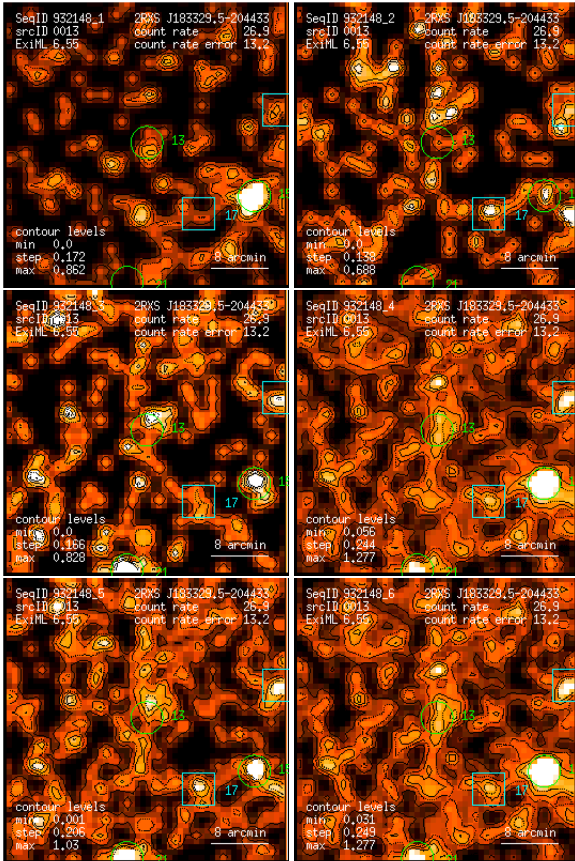
Figure 13: RASS 932148: detection 0013: band rate images, Gaussian filter: (1) PSPC channels 11 – 41, (2) 52 – 90, (3) 91 – 201, (4) 11 – 235, (5) 52 – 201, (6) 11 – 201. Broad band rates in counts/ks. Band rate contour levels in counts/ks/arcmin 2 .
