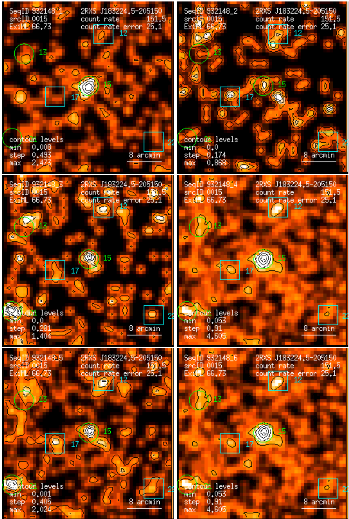
Figure 15: RASS 932148: detection 0015: band rate images, Gaussian filter: (1) PSPC channels 11 – 41, (2) 52 – 90, (3) 91 – 201, (4) 11 – 235, (5) 52 – 201, (6) 11 – 201. Broad band rates in counts/ks. Band rate contour levels in counts/ks/arcmin 2 .
