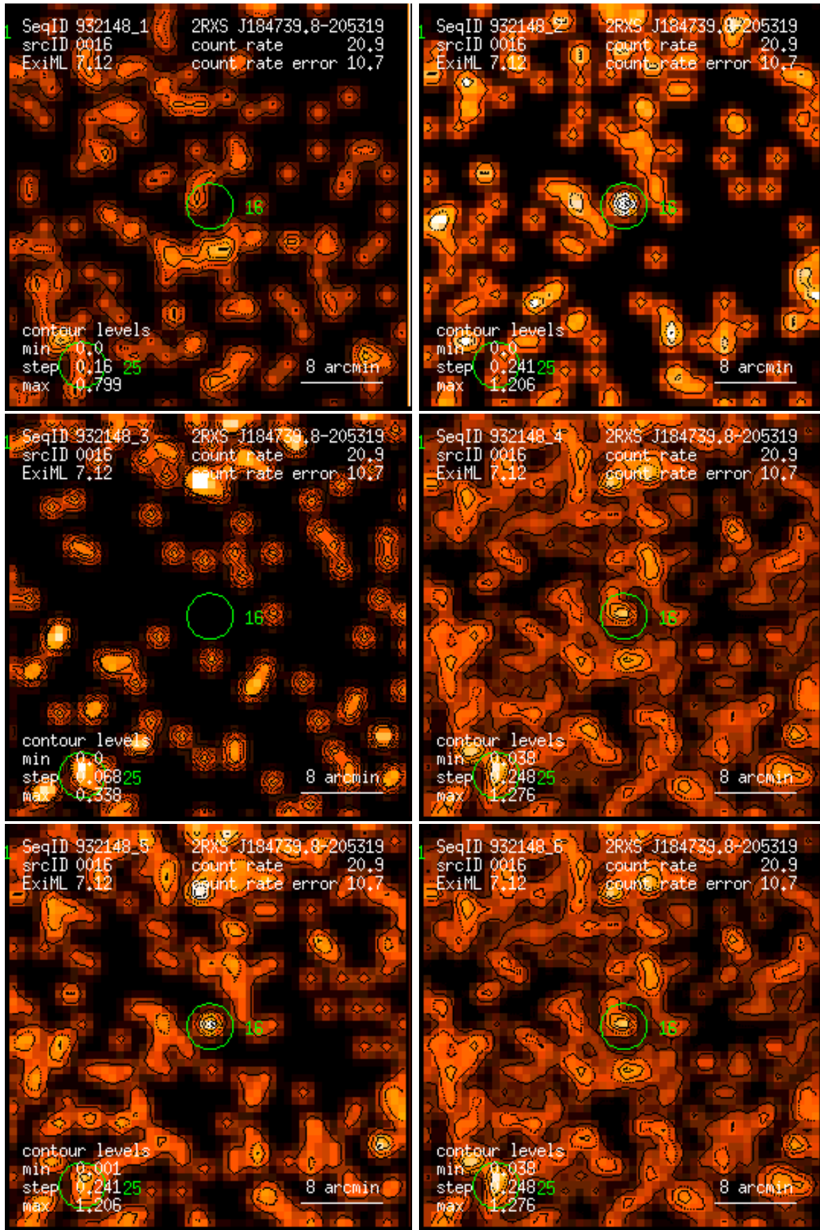
Figure 16: RASS 932148: detection 0016: band rate images, Gaussian filter: (1) PSPC channels 11 – 41, (2) 52 – 90, (3) 91 – 201, (4) 11 – 235, (5) 52 – 201, (6) 11 – 201. Broad band rates in counts/ks. Band rate contour levels in counts/ks/arcmin 2 .
