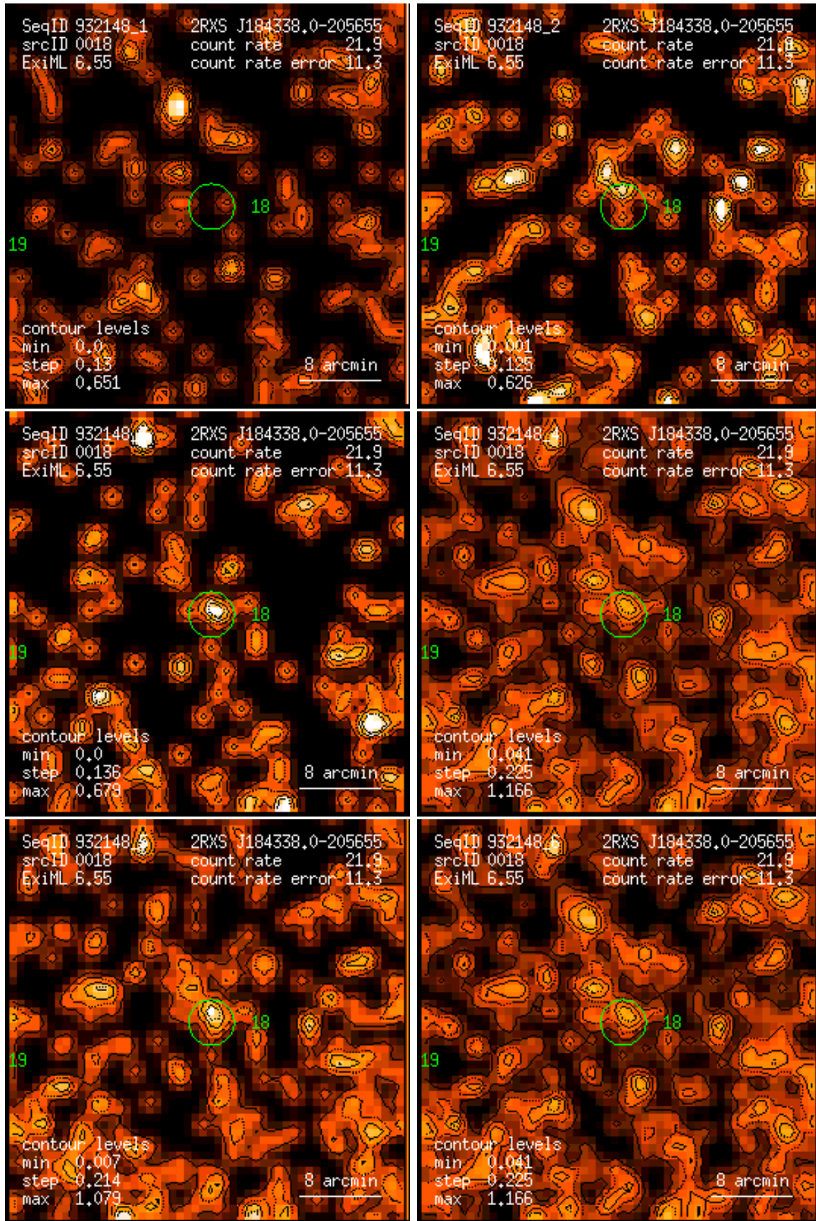
Figure 18: RASS 932148: detection 0018: band rate images, Gaussian filter: (1) PSPC channels 11 – 41, (2) 52 – 90, (3) 91 – 201, (4) 11 – 235, (5) 52 – 201, (6) 11 – 201. Broad band rates in counts/ks. Band rate contour levels in counts/ks/arcmin 2 .
