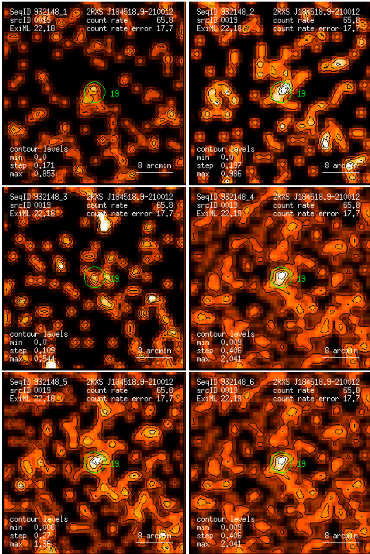
Figure 19: RASS 932148: detection 0019: band rate images, Gaussian filter: (1) PSPC channels 11 – 41, (2) 52 – 90, (3) 91 – 201, (4) 11 – 235, (5) 52 – 201, (6) 11 – 201. Broad band rates in counts/ks. Band rate contour levels in counts/ks/arcmin 2 .
