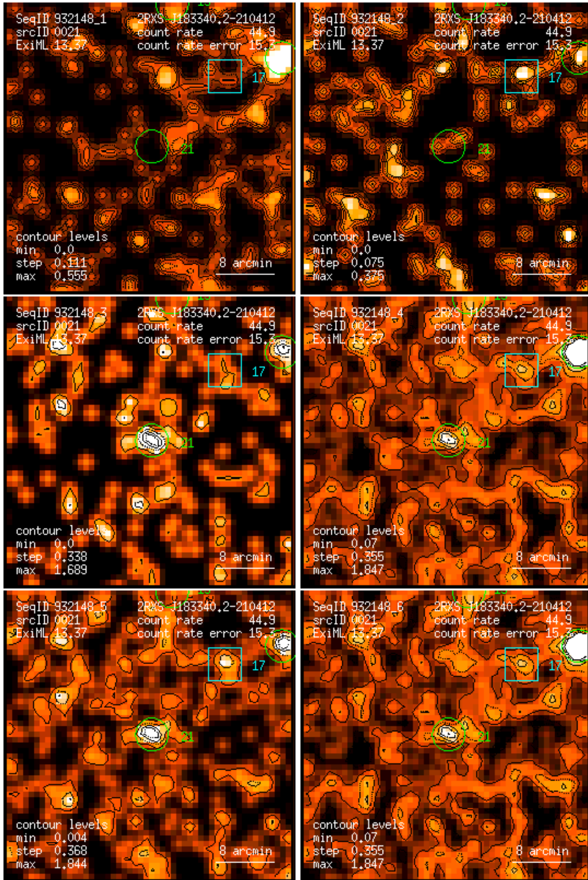
Figure 21: RASS 932148: detection 0021: band rate images, Gaussian filter: (1) PSPC channels 11 – 41, (2) 52 – 90, (3) 91 – 201, (4) 11 – 235, (5) 52 – 201, (6) 11 – 201. Broad band rates in counts/ks. Band rate contour levels in counts/ks/arcmin 2 .
