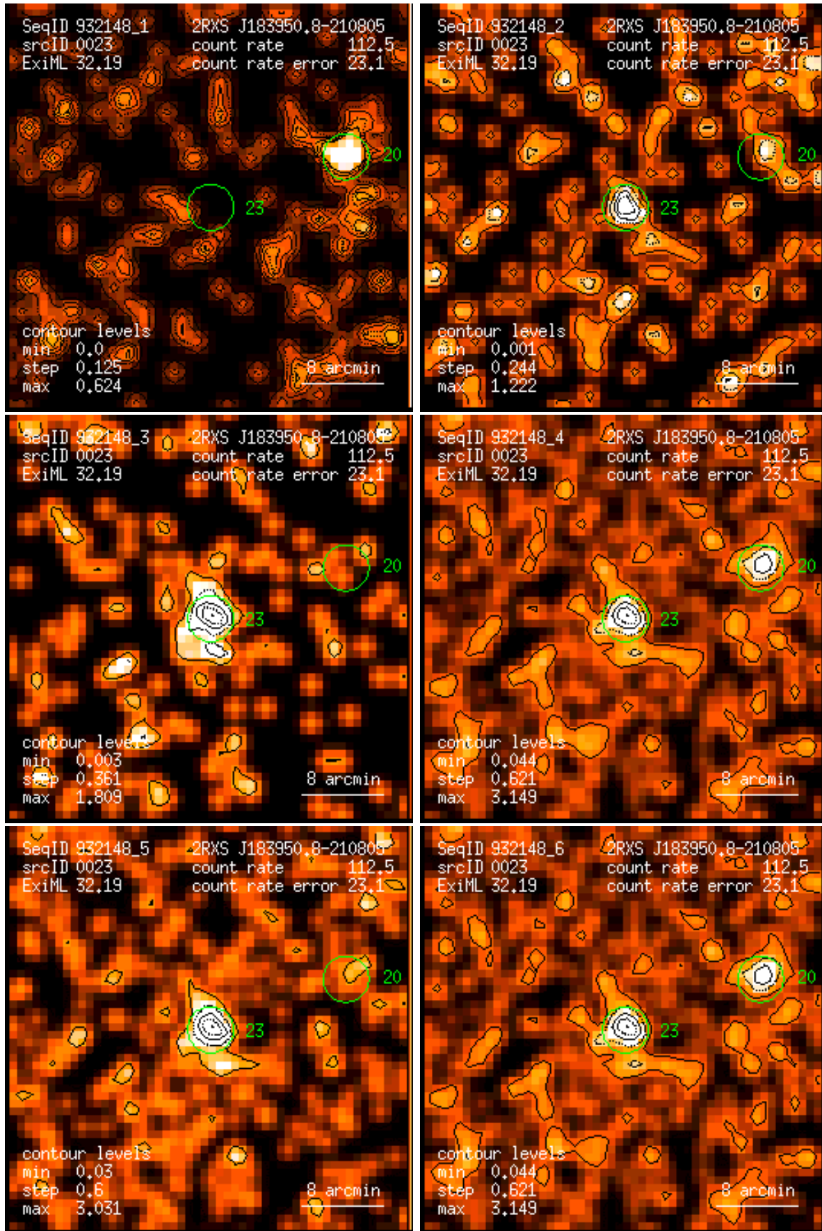
Figure 23: RASS 932148: detection 0023: band rate images, Gaussian filter: (1) PSPC channels 11 – 41, (2) 52 – 90, (3) 91 – 201, (4) 11 – 235, (5) 52 – 201, (6) 11 – 201. Broad band rates in counts/ks. Band rate contour levels in counts/ks/arcmin 2 .
