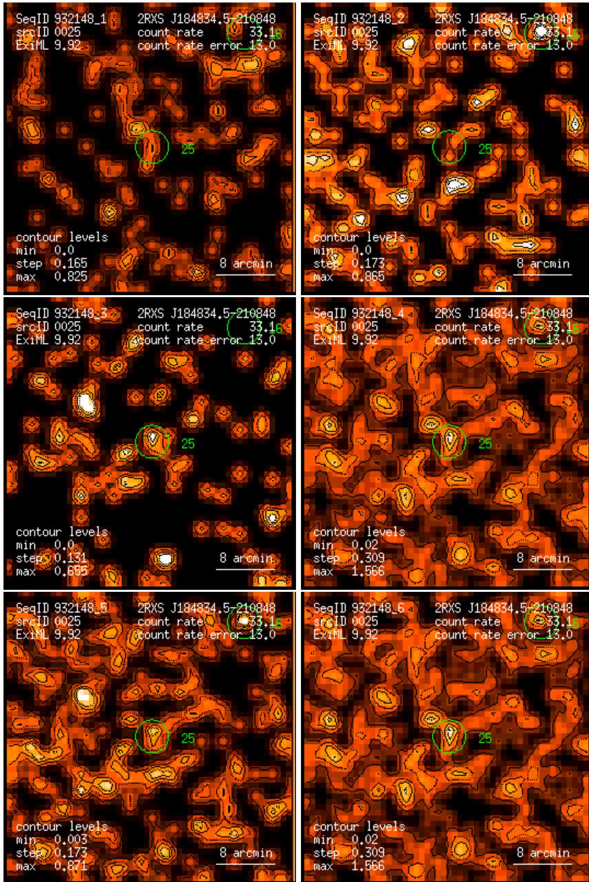
Figure 25: RASS 932148: detection 0025: band rate images, Gaussian filter: (1) PSPC channels 11 – 41, (2) 52 – 90, (3) 91 – 201, (4) 11 – 235, (5) 52 – 201, (6) 11 – 201. Broad band rates in counts/ks. Band rate contour levels in counts/ks/arcmin 2 .
