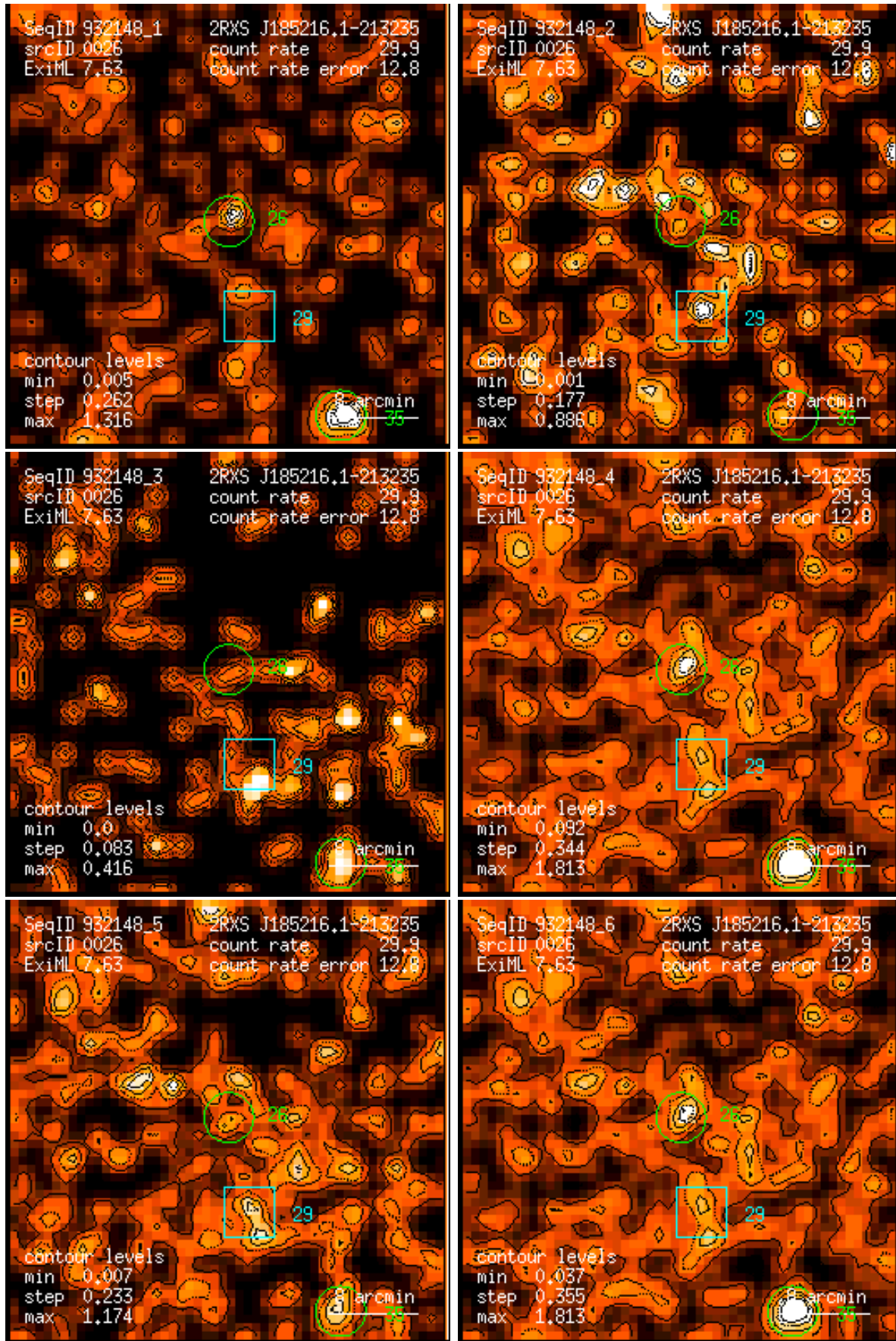
Figure 26: RASS 932148: detection 0026: band rate images, Gaussian filter: (1) PSPC channels 11 – 41, (2) 52 – 90, (3) 91 – 201, (4) 11 – 235, (5) 52 – 201, (6) 11 – 201. Broad band rates in counts/ks. Band rate contour levels in counts/ks/arcmin 2 .
