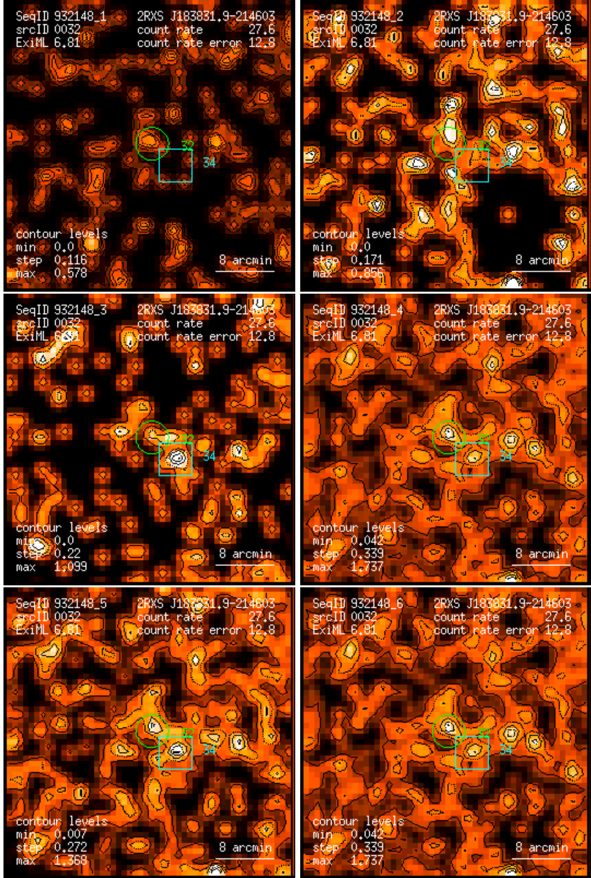
Figure 32: RASS 932148: detection 0032: band rate images, Gaussian filter: (1) PSPC channels 11 – 41, (2) 52 – 90, (3) 91 – 201, (4) 11 – 235, (5) 52 – 201, (6) 11 – 201. Broad band rates in counts/ks. Band rate contour levels in counts/ks/arcmin 2 .
