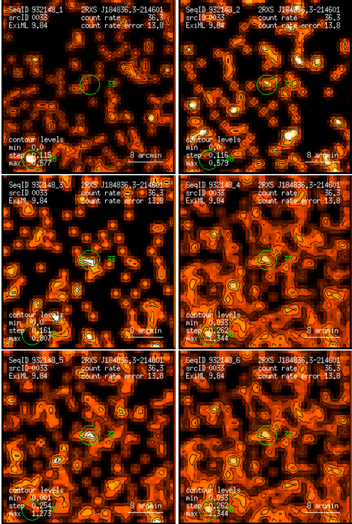
Figure 33: RASS 932148: detection 0033: band rate images, Gaussian filter: (1) PSPC channels 11 – 41, (2) 52 – 90, (3) 91 – 201, (4) 11 – 235, (5) 52 – 201, (6) 11 – 201. Broad band rates in counts/ks. Band rate contour levels in counts/ks/arcmin 2 .
