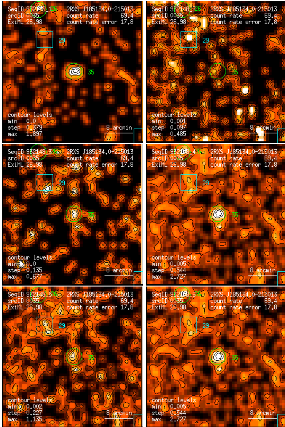
Figure 35: RASS 932148: detection 0035: band rate images, Gaussian filter: (1) PSPC channels 11 – 41, (2) 52 – 90, (3) 91 – 201, (4) 11 – 235, (5) 52 – 201, (6) 11 – 201. Broad band rates in counts/ks. Band rate contour levels in counts/ks/arcmin 2 .
