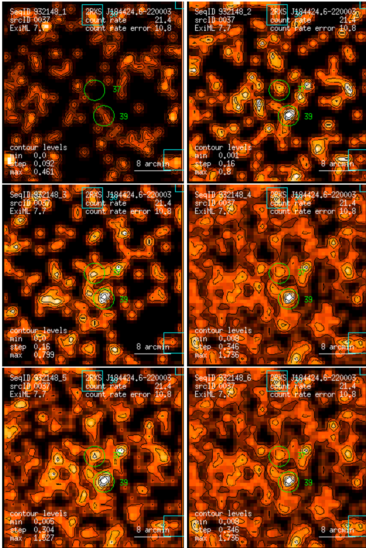
Figure 37: RASS 932148: detection 0037: band rate images, Gaussian filter: (1) PSPC channels 11 – 41, (2) 52 – 90, (3) 91 – 201, (4) 11 – 235, (5) 52 – 201, (6) 11 – 201. Broad band rates in counts/ks. Band rate contour levels in counts/ks/arcmin 2 .
