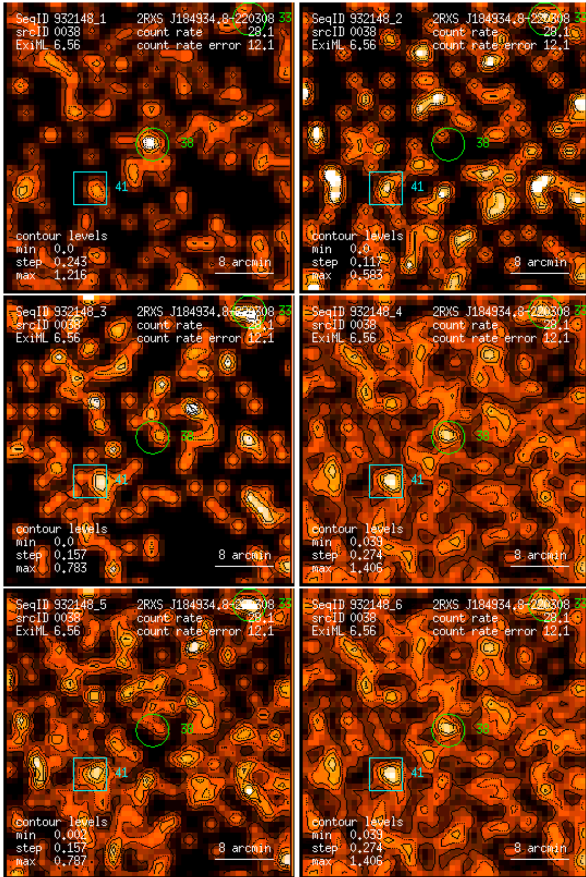
Figure 38: RASS 932148: detection 0038: band rate images, Gaussian filter: (1) PSPC channels 11 – 41, (2) 52 – 90, (3) 91 – 201, (4) 11 – 235, (5) 52 – 201, (6) 11 – 201. Broad band rates in counts/ks. Band rate contour levels in counts/ks/arcmin 2 .
