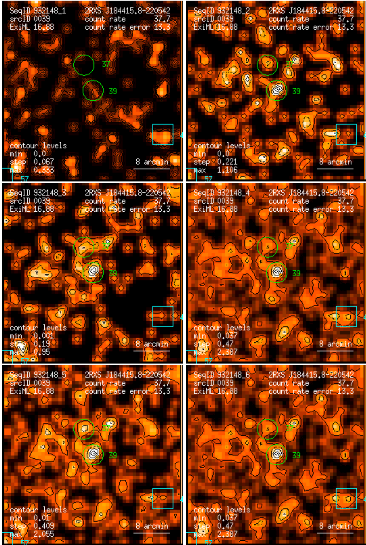
Figure 39: RASS 932148: detection 0039: band rate images, Gaussian filter: (1) PSPC channels 11 – 41, (2) 52 – 90, (3) 91 – 201, (4) 11 – 235, (5) 52 – 201, (6) 11 – 201. Broad band rates in counts/ks. Band rate contour levels in counts/ks/arcmin 2 .
