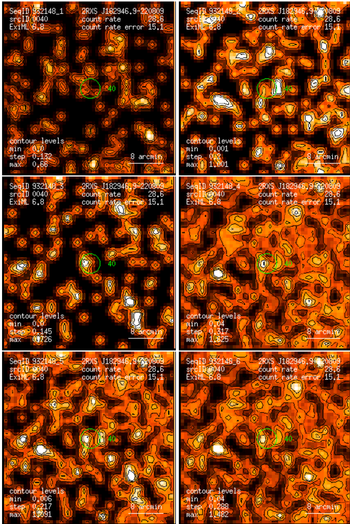
Figure 40: RASS 932148: detection 0040: band rate images, Gaussian filter: (1) PSPC channels 11 – 41, (2) 52 – 90, (3) 91 – 201, (4) 11 – 235, (5) 52 – 201, (6) 11 – 201. Broad band rates in counts/ks. Band rate contour levels in counts/ks/arcmin 2 .
