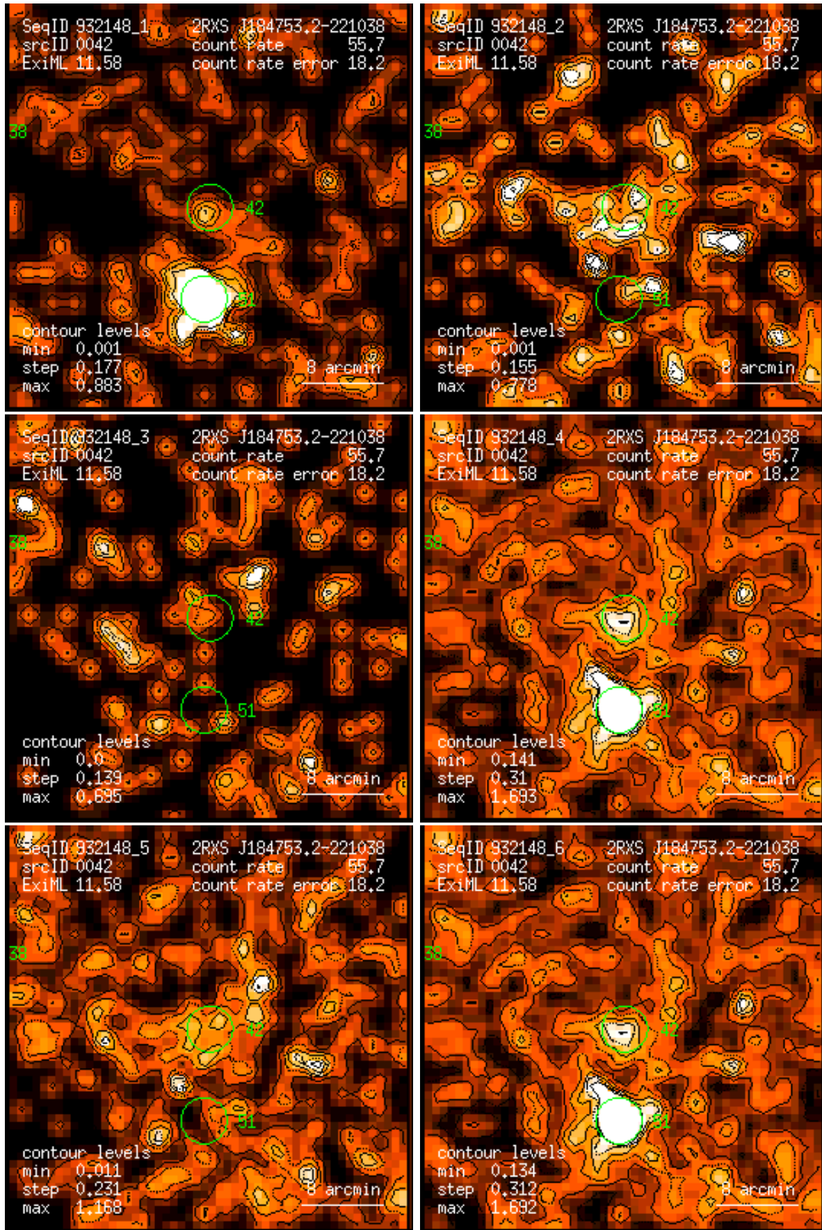
Figure 42: RASS 932148: detection 0042: band rate images, Gaussian filter: (1) PSPC channels 11 – 41, (2) 52 – 90, (3) 91 – 201, (4) 11 – 235, (5) 52 – 201, (6) 11 – 201. Broad band rates in counts/ks. Band rate contour levels in counts/ks/arcmin 2 .
