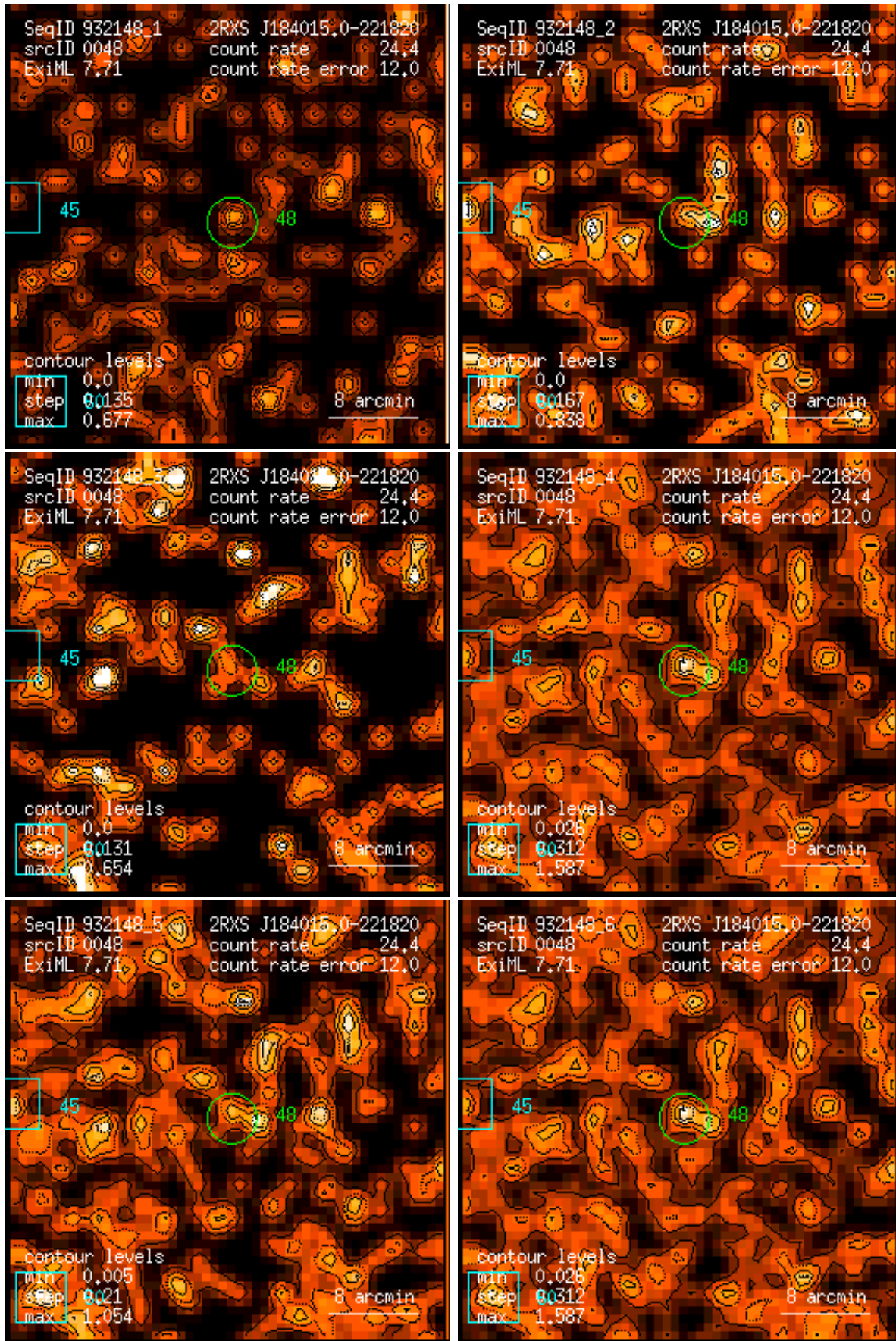
Figure 48: RASS 932148: detection 0048: band rate images, Gaussian filter: (1) PSPC channels 11 – 41, (2) 52 – 90, (3) 91 – 201, (4) 11 – 235, (5) 52 – 201, (6) 11 – 201. Broad band rates in counts/ks. Band rate contour levels in counts/ks/arcmin 2 .
