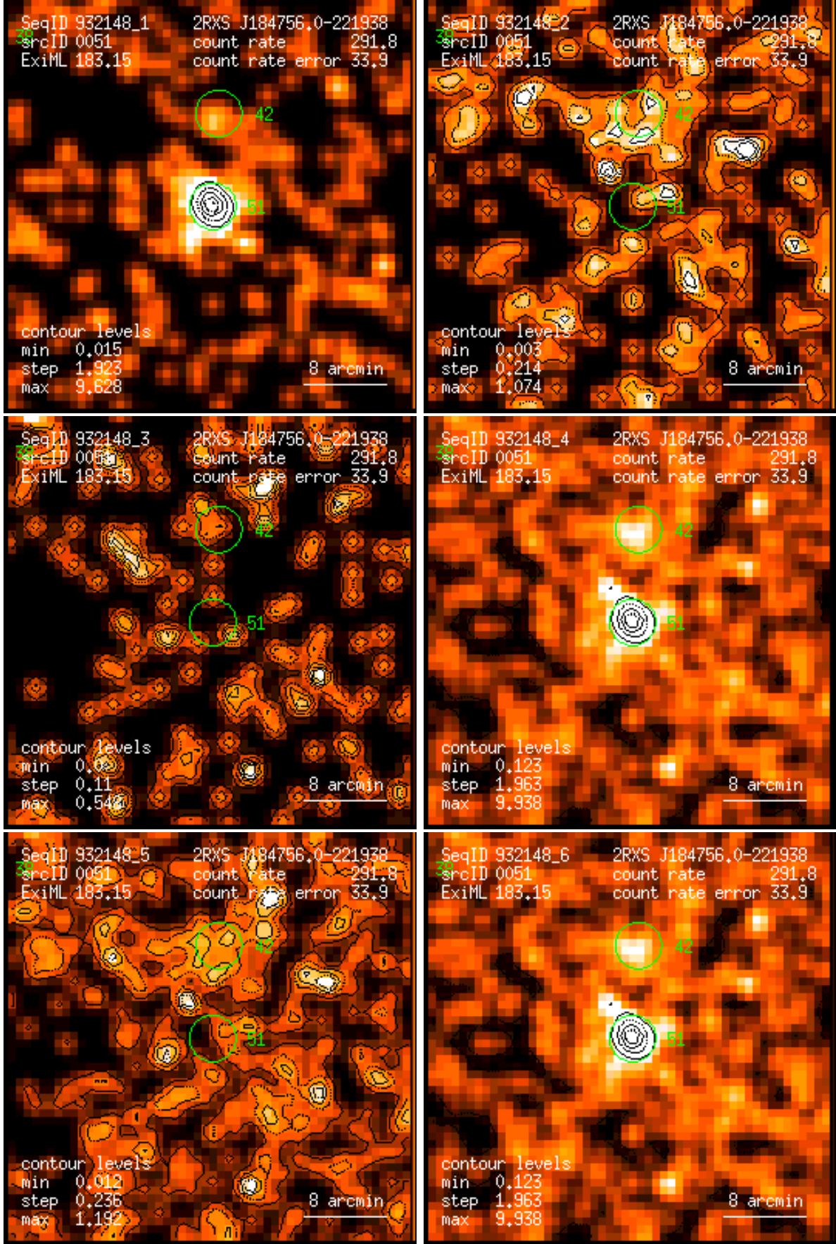
Figure 51: RASS 932148: detection 0051: band rate images, Gaussian filter: (1) PSPC channels 11 – 41, (2) 52 – 90, (3) 91 – 201, (4) 11 – 235, (5) 52 – 201, (6) 11 – 201. Broad band rates in counts/ks. Band rate contour levels in counts/ks/arcmin 2 .
