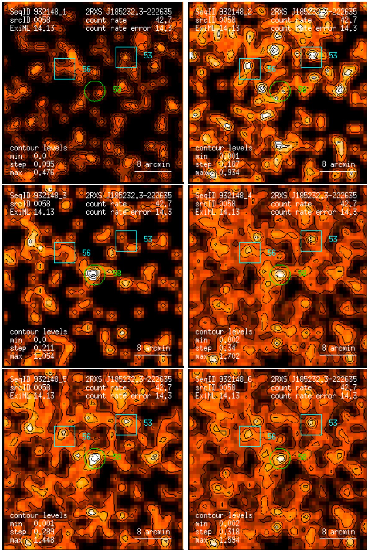
Figure 58: RASS 932148: detection 0058: band rate images, Gaussian filter: (1) PSPC channels 11 – 41, (2) 52 – 90, (3) 91 – 201, (4) 11 – 235, (5) 52 – 201, (6) 11 – 201. Broad band rates in counts/ks. Band rate contour levels in counts/ks/arcmin 2 .
