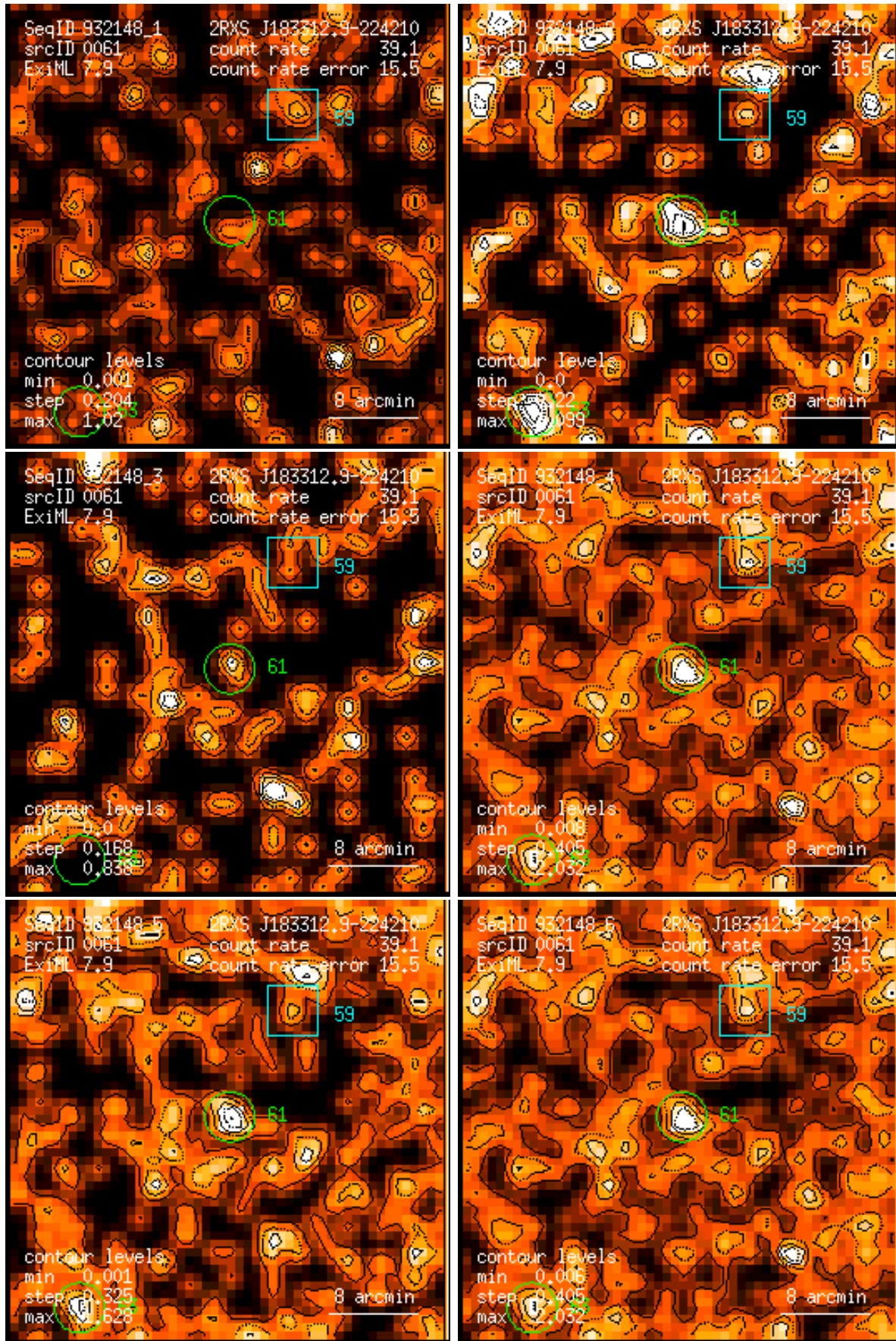
Figure 61: RASS 932148: detection 0061: band rate images, Gaussian filter: (1) PSPC channels 11 – 41, (2) 52 – 90, (3) 91 – 201, (4) 11 – 235, (5) 52 – 201, (6) 11 – 201. Broad band rates in counts/ks. Band rate contour levels in counts/ks/arcmin 2 .
