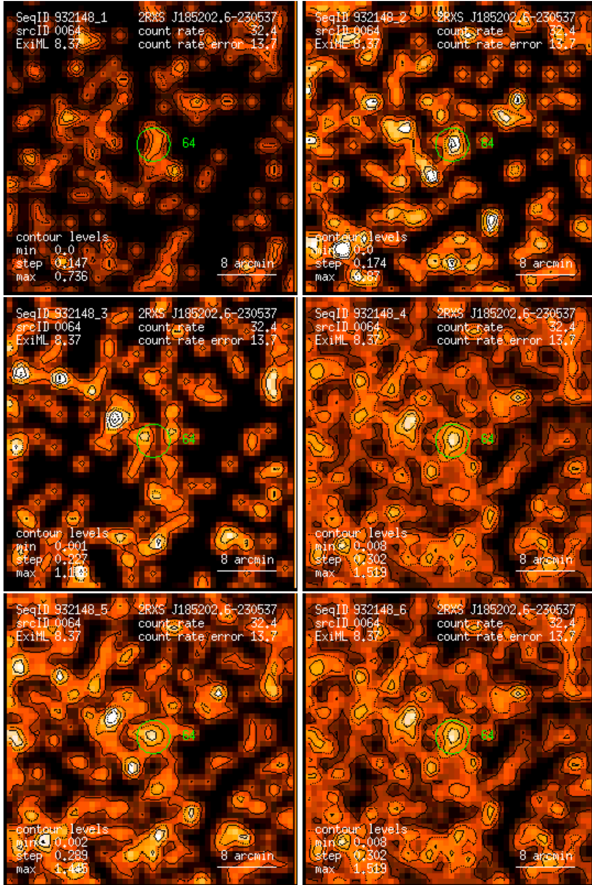
Figure 64: RASS 932148: detection 0064: band rate images, Gaussian filter: (1) PSPC channels 11 – 41, (2) 52 – 90, (3) 91 – 201, (4) 11 – 235, (5) 52 – 201, (6) 11 – 201. Broad band rates in counts/ks. Band rate contour levels in counts/ks/arcmin 2 .
