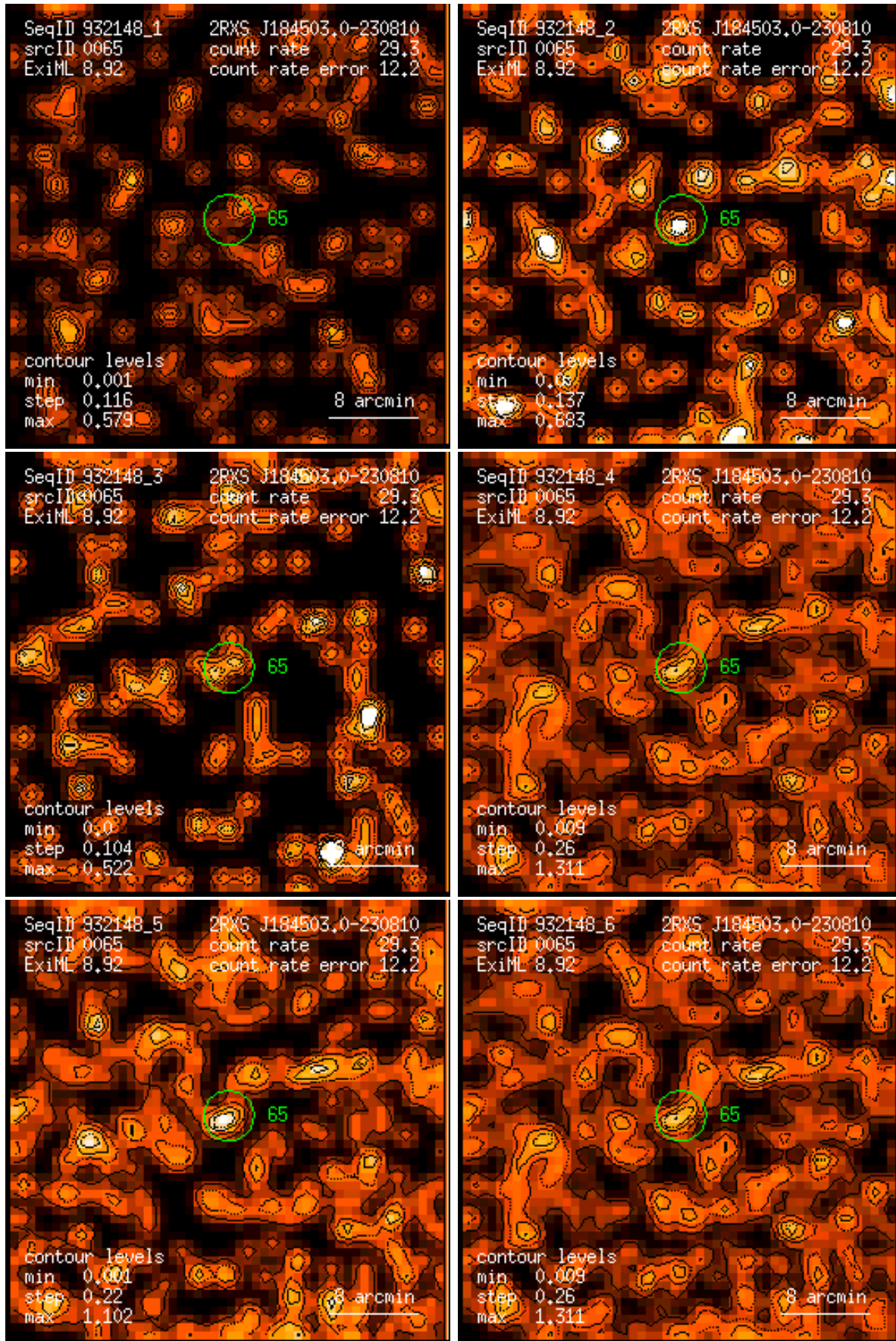
Figure 65: RASS 932148: detection 0065: band rate images, Gaussian filter: (1) PSPC channels 11 – 41, (2) 52 – 90, (3) 91 – 201, (4) 11 – 235, (5) 52 – 201, (6) 11 – 201. Broad band rates in counts/ks. Band rate contour levels in counts/ks/arcmin 2 .
