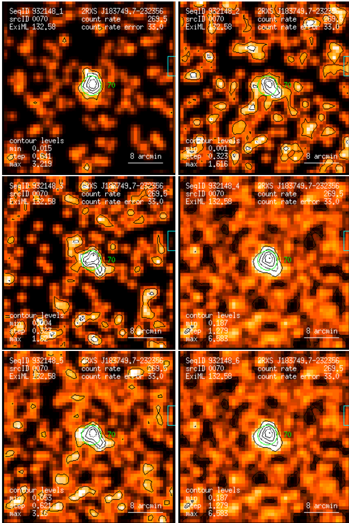
Figure 70: RASS 932148: detection 0070: band rate images, Gaussian filter: (1) PSPC channels 11 – 41, (2) 52 – 90, (3) 91 – 201, (4) 11 – 235, (5) 52 – 201, (6) 11 – 201. Broad band rates in counts/ks. Band rate contour levels in counts/ks/arcmin 2 .
