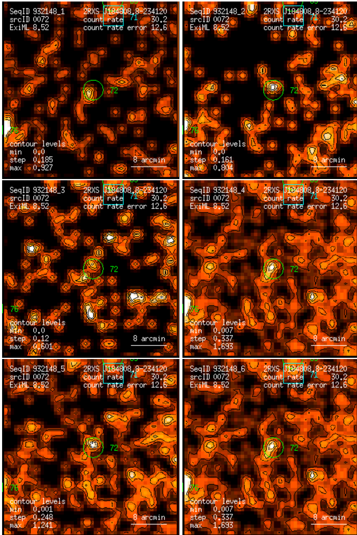
Figure 72: RASS 932148: detection 0072: band rate images, Gaussian filter: (1) PSPC channels 11 – 41, (2) 52 – 90, (3) 91 – 201, (4) 11 – 235, (5) 52 – 201, (6) 11 – 201. Broad band rates in counts/ks. Band rate contour levels in counts/ks/arcmin 2 .
