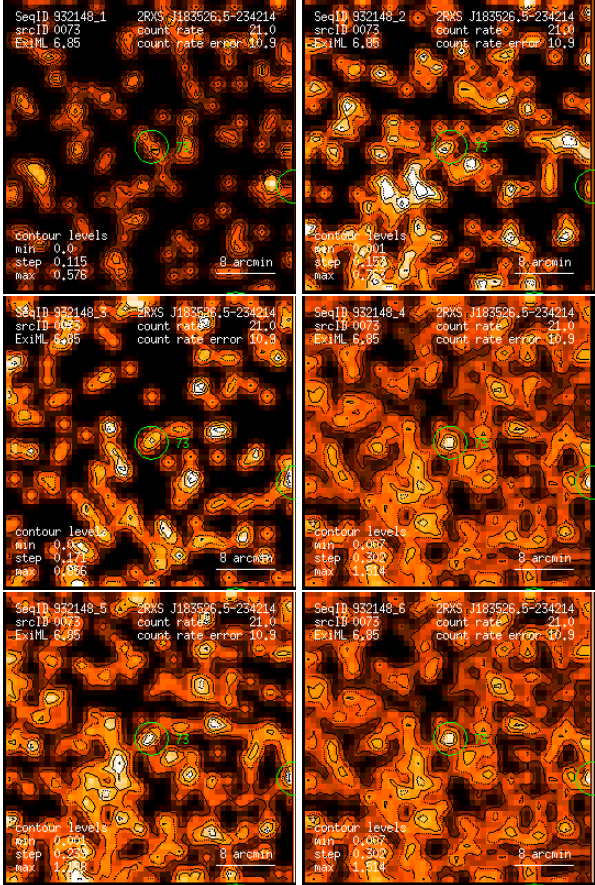
Figure 73: RASS 932148: detection 0073: band rate images, Gaussian filter: (1) PSPC channels 11 – 41, (2) 52 – 90, (3) 91 – 201, (4) 11 – 235, (5) 52 – 201, (6) 11 – 201. Broad band rates in counts/ks. Band rate contour levels in counts/ks/arcmin 2 .
