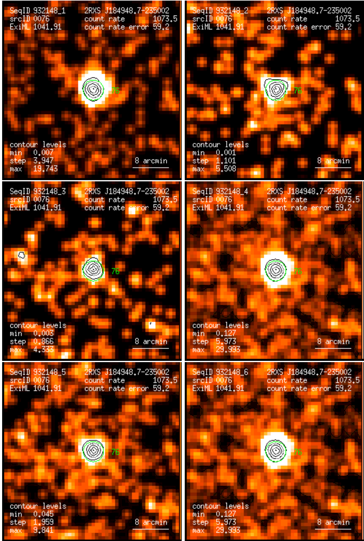
Figure 76: RASS 932148: detection 0076: band rate images, Gaussian filter: (1) PSPC channels 11 – 41, (2) 52 – 90, (3) 91 – 201, (4) 11 – 235, (5) 52 – 201, (6) 11 – 201. Broad band rates in counts/ks. Band rate contour levels in counts/ks/arcmin 2 .
