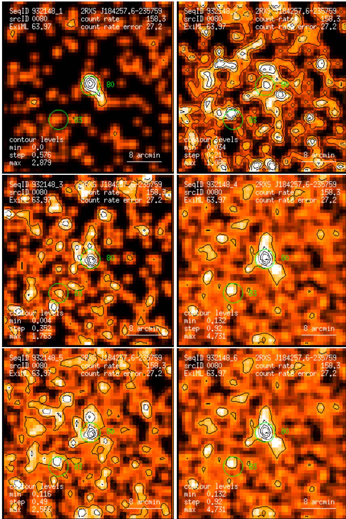
Figure 80: RASS 932148: detection 0080: band rate images, Gaussian filter: (1) PSPC channels 11 – 41, (2) 52 – 90, (3) 91 – 201, (4) 11 – 235, (5) 52 – 201, (6) 11 – 201. Broad band rates in counts/ks. Band rate contour levels in counts/ks/arcmin 2 .
