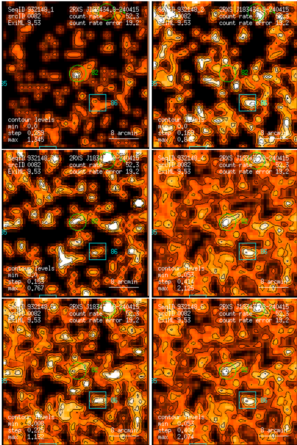
Figure 82: RASS 932148: detection 0082: band rate images, Gaussian filter: (1) PSPC channels 11 – 41, (2) 52 – 90, (3) 91 – 201, (4) 11 – 235, (5) 52 – 201, (6) 11 – 201. Broad band rates in counts/ks. Band rate contour levels in counts/ks/arcmin 2 .
