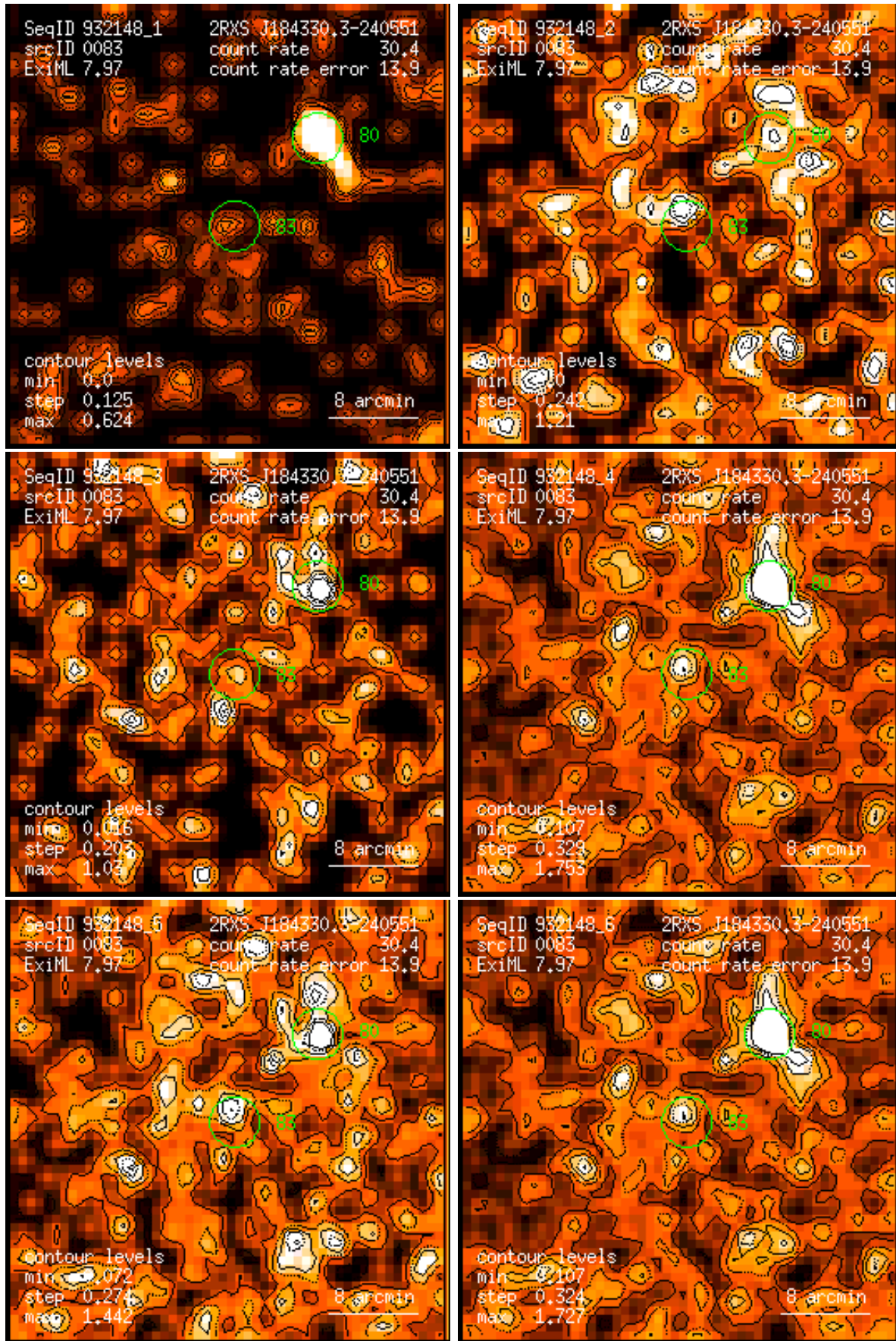
Figure 83: RASS 932148: detection 0083: band rate images, Gaussian filter: (1) PSPC channels 11 – 41, (2) 52 – 90, (3) 91 – 201, (4) 11 – 235, (5) 52 – 201, (6) 11 – 201. Broad band rates in counts/ks. Band rate contour levels in counts/ks/arcmin 2 .
