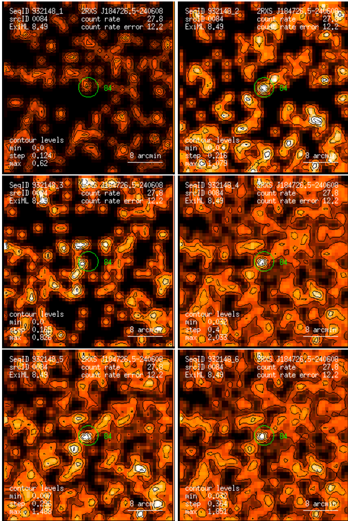
Figure 84: RASS 932148: detection 0084: band rate images, Gaussian filter: (1) PSPC channels 11 – 41, (2) 52 – 90, (3) 91 – 201, (4) 11 – 235, (5) 52 – 201, (6) 11 – 201. Broad band rates in counts/ks. Band rate contour levels in counts/ks/arcmin 2 .
