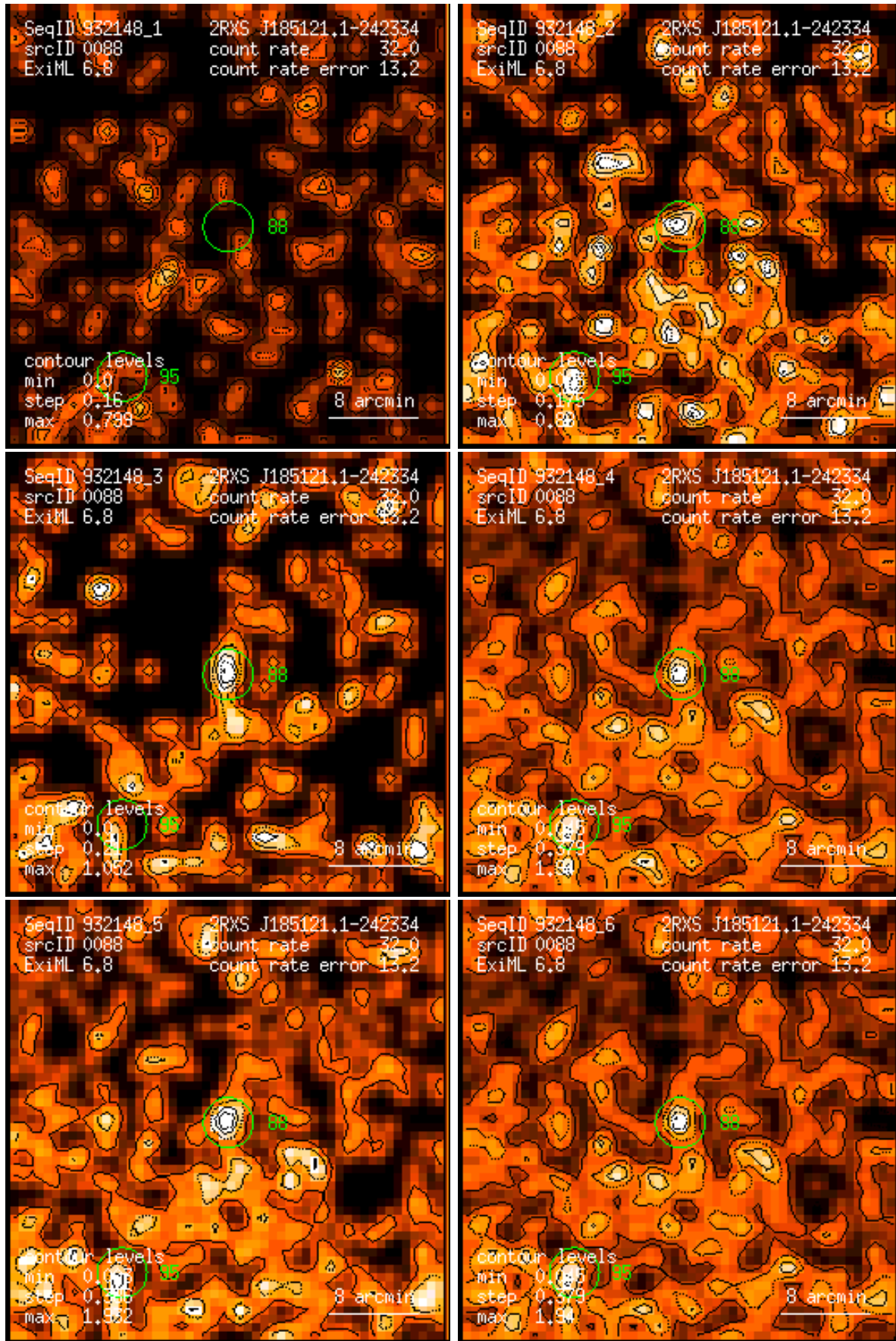
Figure 88: RASS 932148: detection 0088: band rate images, Gaussian filter: (1) PSPC channels 11 – 41, (2) 52 – 90, (3) 91 – 201, (4) 11 – 235, (5) 52 – 201, (6) 11 – 201. Broad band rates in counts/ks. Band rate contour levels in counts/ks/arcmin 2 .
