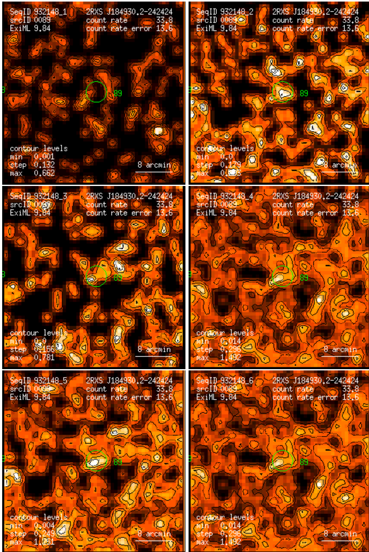
Figure 89: RASS 932148: detection 0089: band rate images, Gaussian filter: (1) PSPC channels 11 – 41, (2) 52 – 90, (3) 91 – 201, (4) 11 – 235, (5) 52 – 201, (6) 11 – 201. Broad band rates in counts/ks. Band rate contour levels in counts/ks/arcmin 2 .
