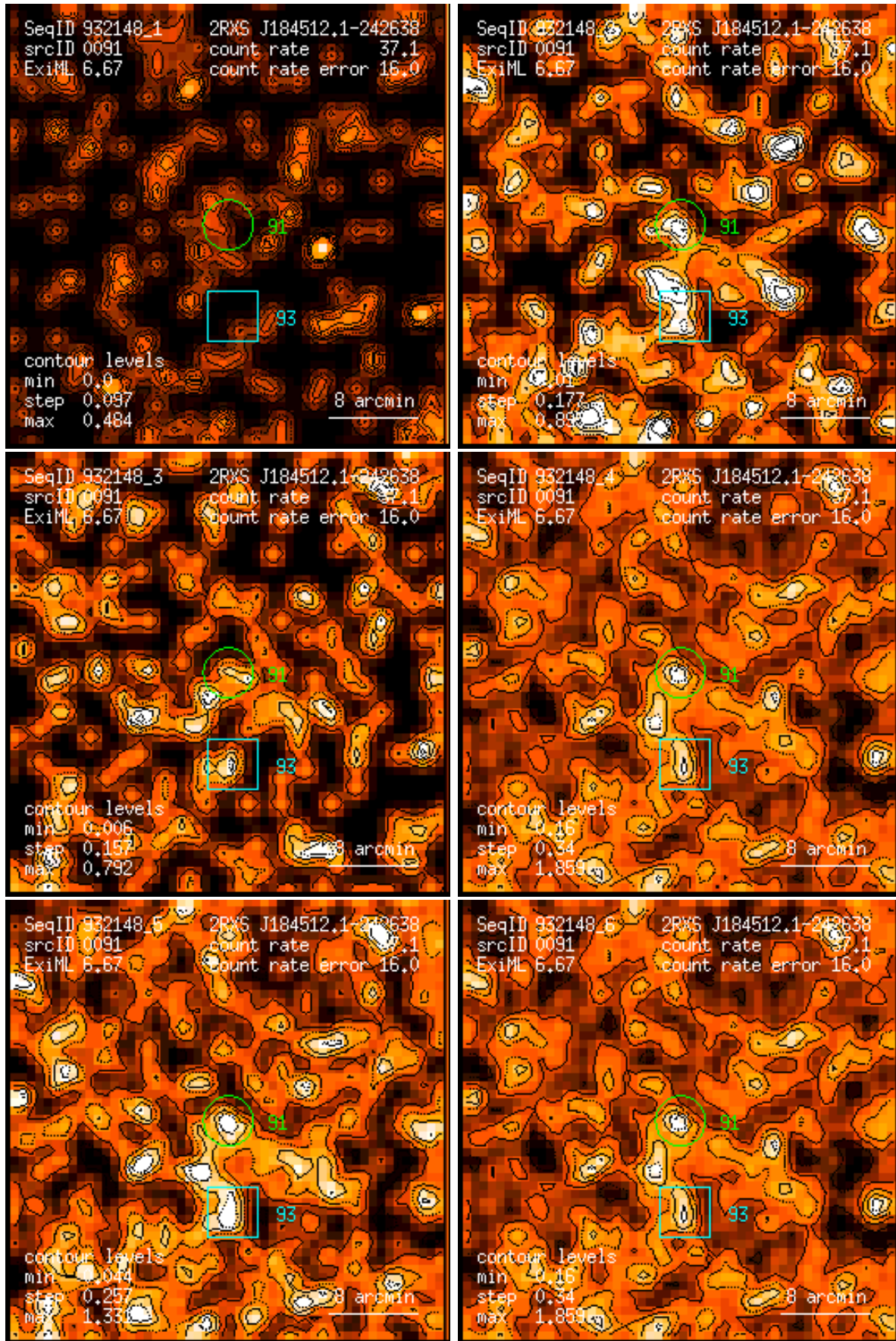
Figure 91: RASS 932148: detection 0091: band rate images, Gaussian filter: (1) PSPC channels 11 – 41, (2) 52 – 90, (3) 91 – 201, (4) 11 – 235, (5) 52 – 201, (6) 11 – 201. Broad band rates in counts/ks. Band rate contour levels in counts/ks/arcmin 2 .
