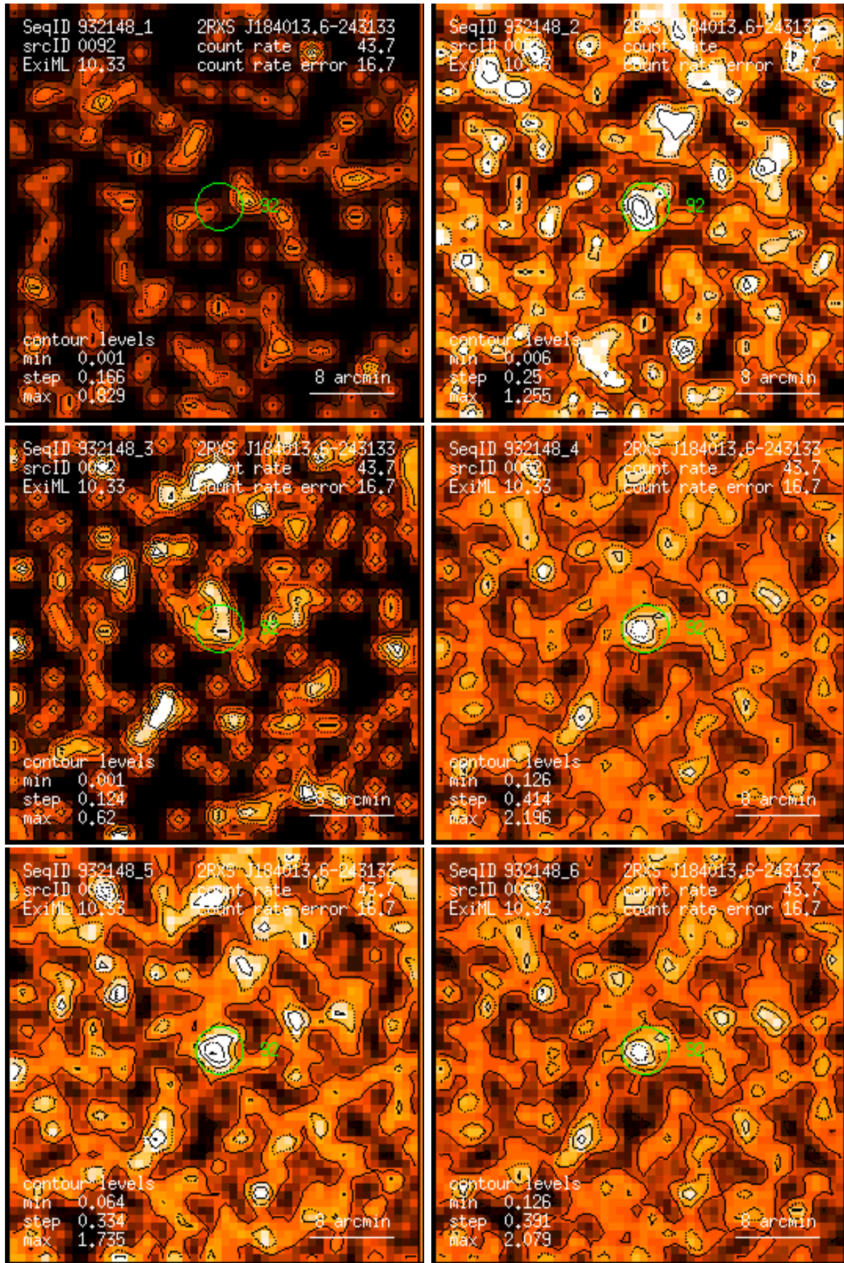
Figure 92: RASS 932148: detection 0092: band rate images, Gaussian filter: (1) PSPC channels 11 – 41, (2) 52 – 90, (3) 91 – 201, (4) 11 – 235, (5) 52 – 201, (6) 11 – 201. Broad band rates in counts/ks. Band rate contour levels in counts/ks/arcmin 2 .
