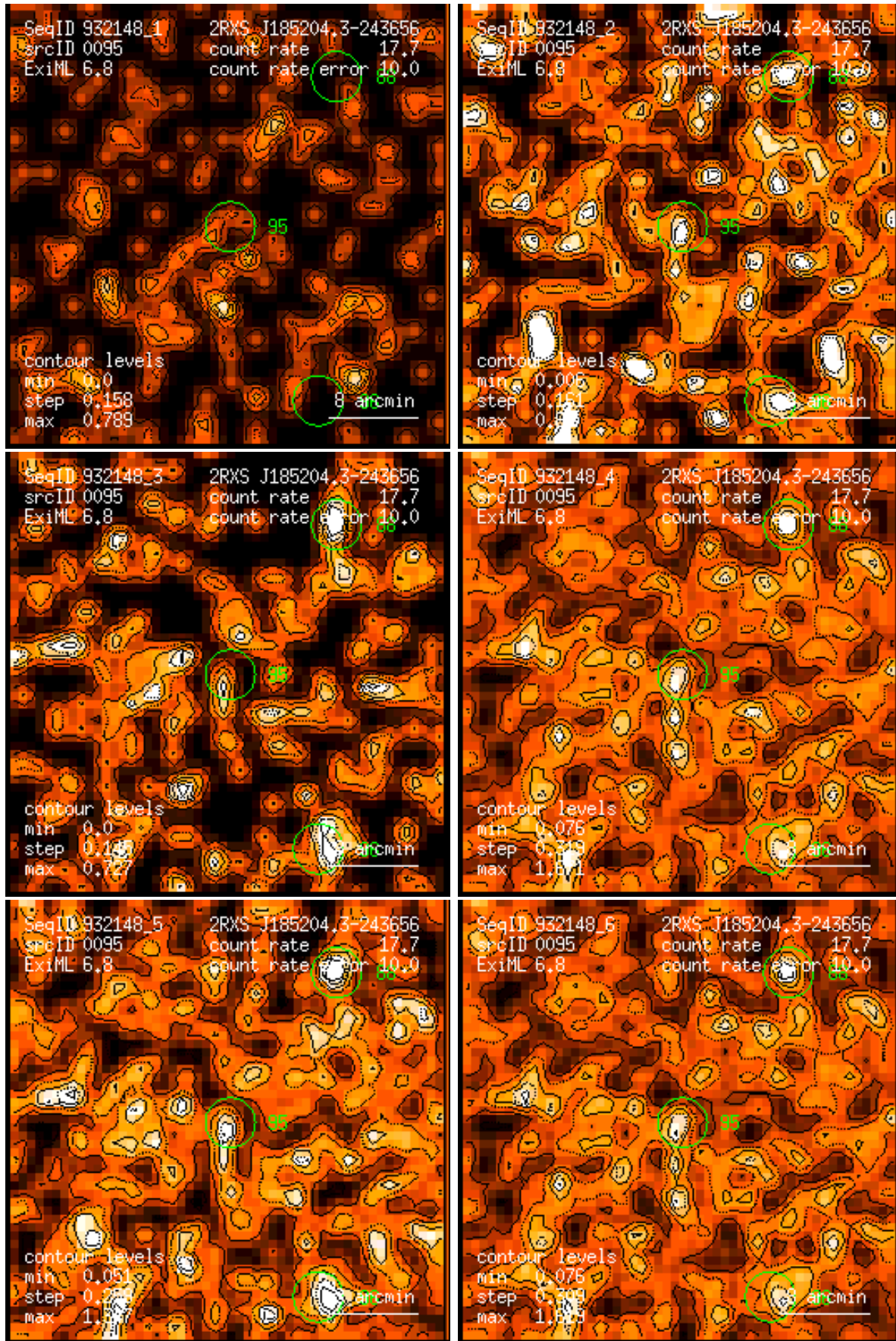
Figure 95: RASS 932148: detection 0095: band rate images, Gaussian filter: (1) PSPC channels 11 – 41, (2) 52 – 90, (3) 91 – 201, (4) 11 – 235, (5) 52 – 201, (6) 11 – 201. Broad band rates in counts/ks. Band rate contour levels in counts/ks/arcmin 2 .
