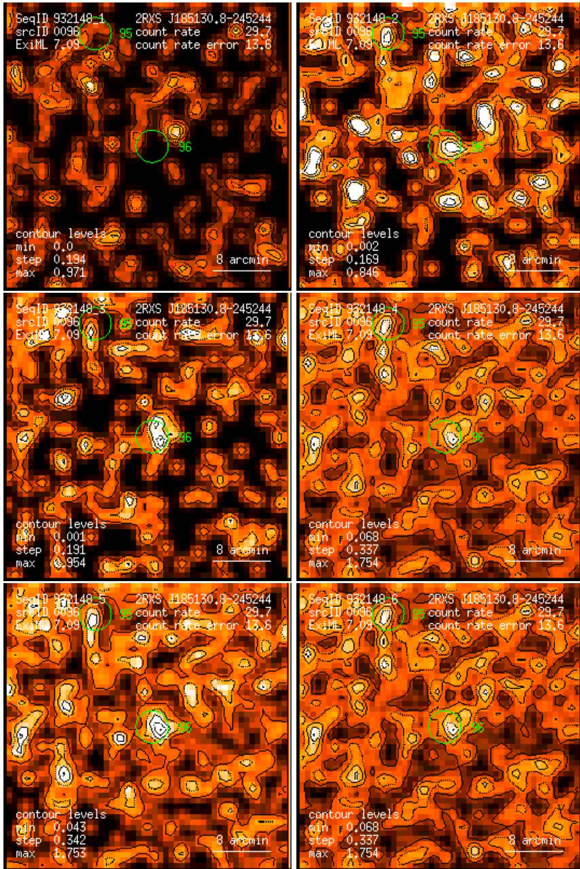
Figure 96: RASS 932148: detection 0096: band rate images, Gaussian filter: (1) PSPC channels 11 – 41, (2) 52 – 90, (3) 91 – 201, (4) 11 – 235, (5) 52 – 201, (6) 11 – 201. Broad band rates in counts/ks. Band rate contour levels in counts/ks/arcmin 2 .
