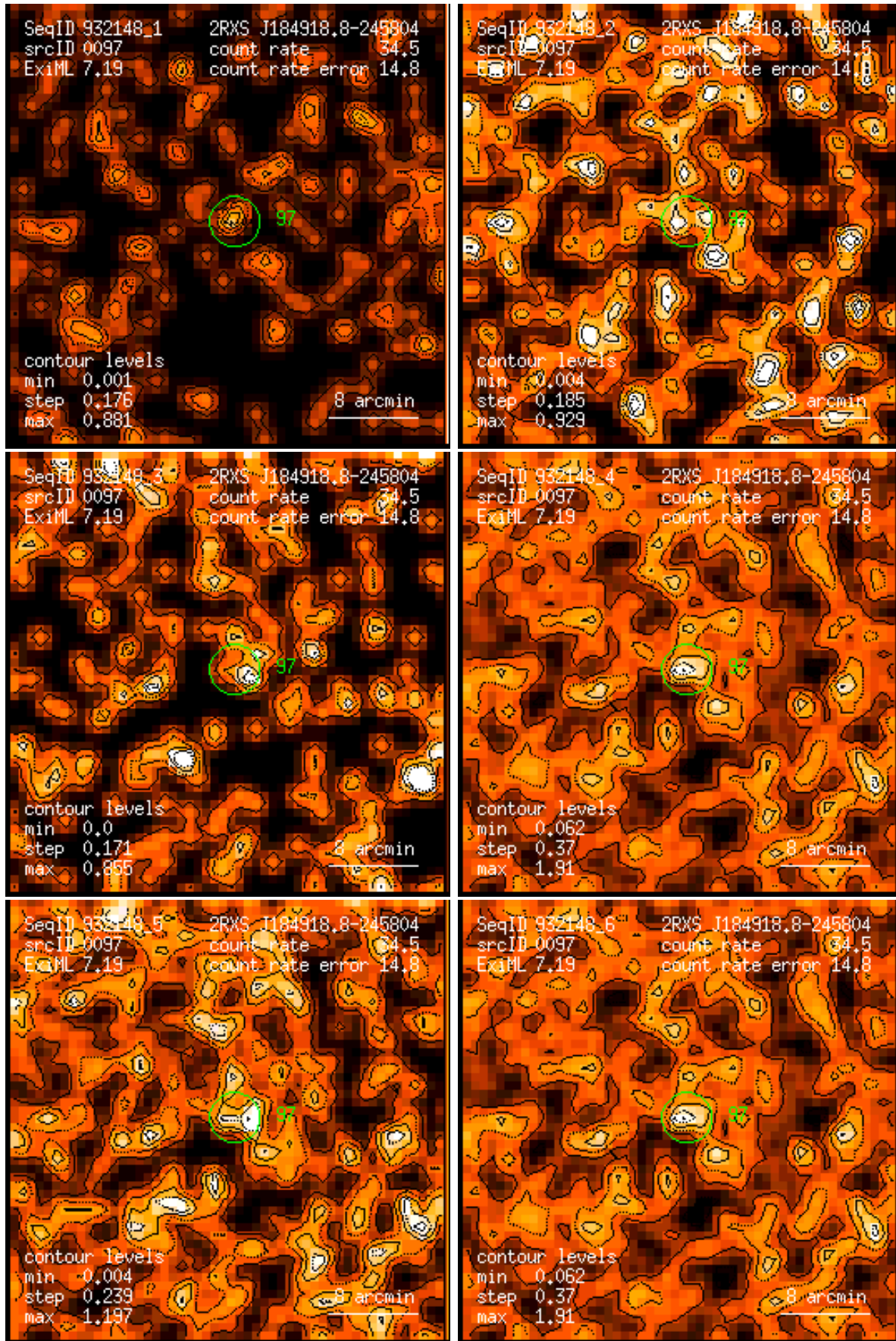
Figure 97: RASS 932148: detection 0097: band rate images, Gaussian filter: (1) PSPC channels 11 – 41, (2) 52 – 90, (3) 91 – 201, (4) 11 – 235, (5) 52 – 201, (6) 11 – 201. Broad band rates in counts/ks. Band rate contour levels in counts/ks/arcmin 2 .
