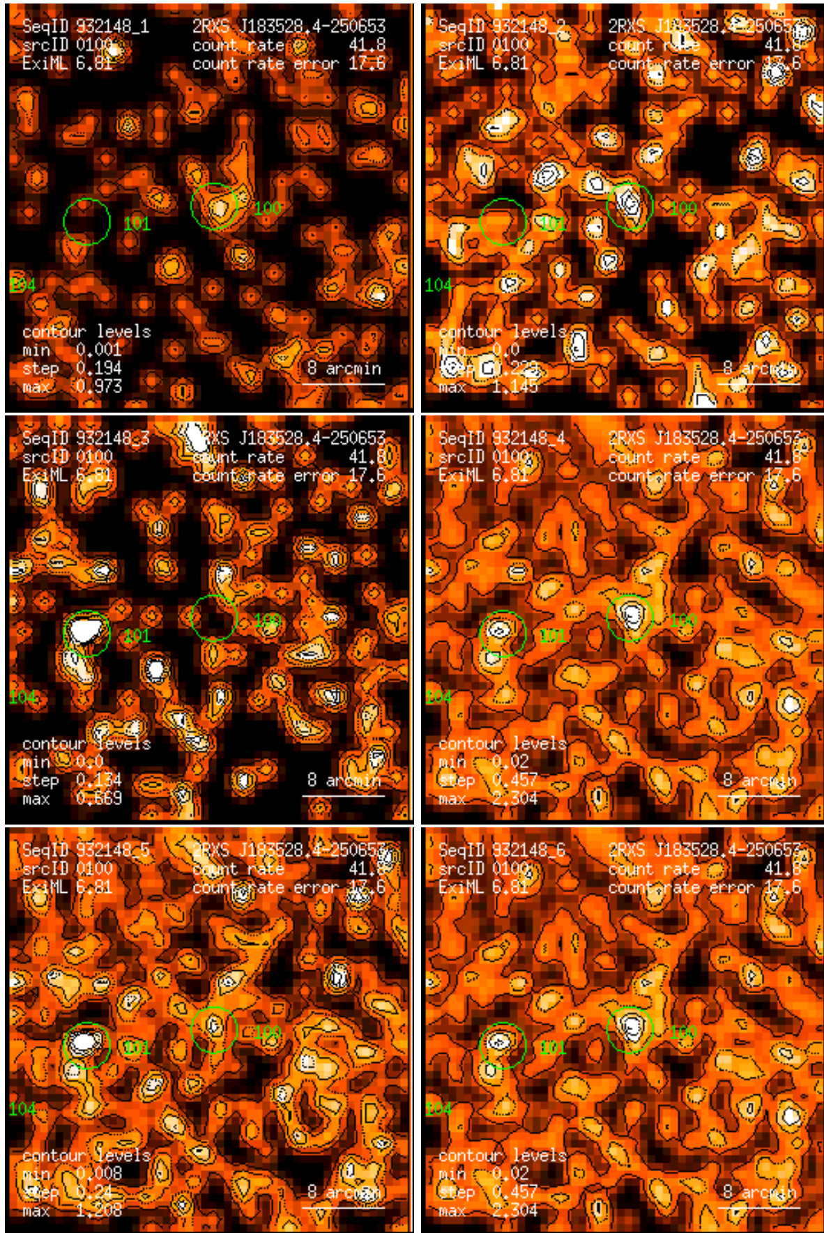
Figure 100: RASS 932148: detection 0100: band rate images, Gaussian filter: (1) PSPC channels 11 – 41, (2) 52 – 90, (3) 91 – 201, (4) 11 – 235, (5) 52 – 201, (6) 11 – 201. Broad band rates in counts/ks. Band rate contour levels in counts/ks/arcmin 2 .
