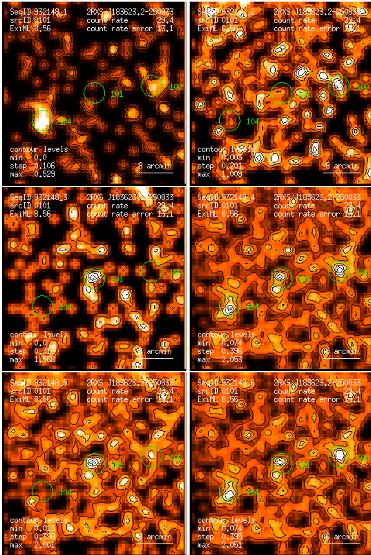
Figure 101: RASS 932148: detection 0101: band rate images, Gaussian filter: (1) PSPC channels 11 – 41, (2) 52 – 90, (3) 91 – 201, (4) 11 – 235, (5) 52 – 201, (6) 11 – 201. Broad band rates in counts/ks. Band rate contour levels in counts/ks/arcmin 2 .
