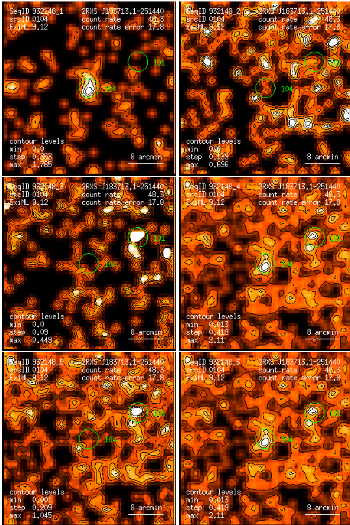
Figure 104: RASS 932148: detection 0104: band rate images, Gaussian filter: (1) PSPC channels 11 – 41, (2) 52 – 90, (3) 91 – 201, (4) 11 – 235, (5) 52 – 201, (6) 11 – 201. Broad band rates in counts/ks. Band rate contour levels in counts/ks/arcmin 2 .
