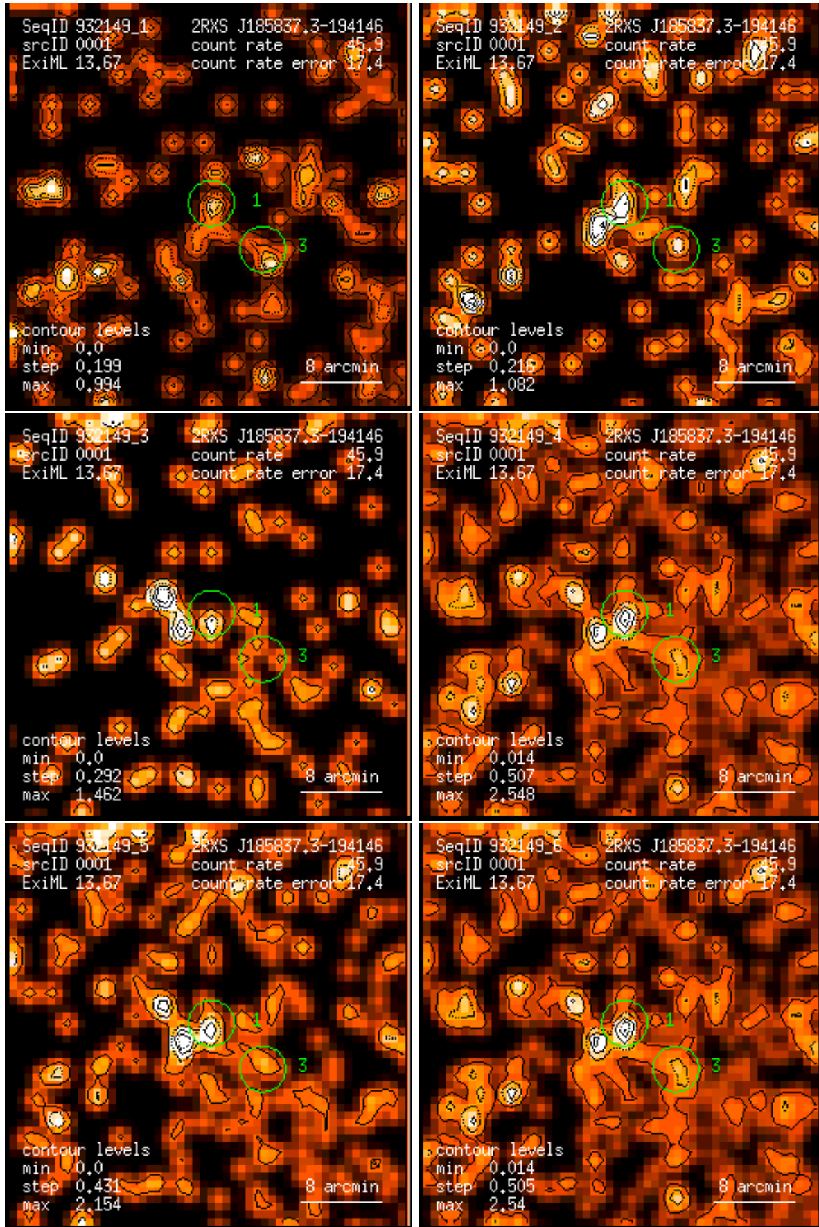
Figure 1: RASS 932149: detection 0001: band rate images, Gaussian filter: (1) PSPC channels 11 – 41, (2) 52 – 90, (3) 91 – 201, (4) 11 – 235, (5) 52 – 201, (6) 11 – 201. Broad band rates in counts/ks. Band rate contour levels in counts/ks/arcmin 2 .
