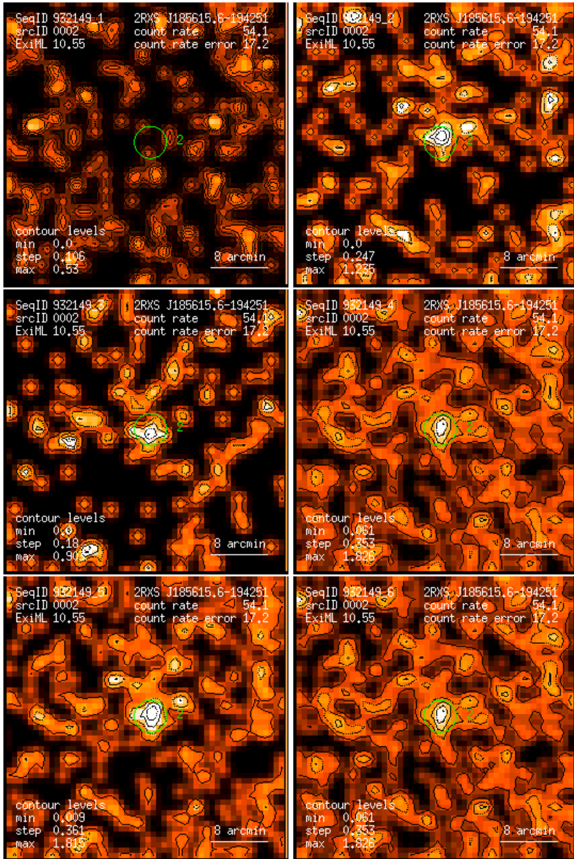
Figure 2: RASS 932149: detection 0002: band rate images, Gaussian filter: (1) PSPC channels 11 – 41, (2) 52 – 90, (3) 91 – 201, (4) 11 – 235, (5) 52 – 201, (6) 11 – 201. Broad band rates in counts/ks. Band rate contour levels in counts/ks/arcmin 2 .
