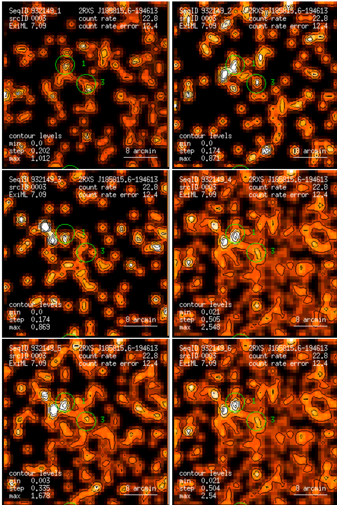
Figure 3: RASS 932149: detection 0003: band rate images, Gaussian filter: (1) PSPC channels 11 – 41, (2) 52 – 90, (3) 91 – 201, (4) 11 – 235, (5) 52 – 201, (6) 11 – 201. Broad band rates in counts/ks. Band rate contour levels in counts/ks/arcmin 2 .
